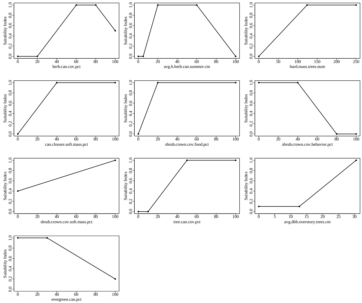
Figure 1. Suitability index graphs for variables included in the easternwildturkeyForestHardDBH38.1cm model in ecores.
